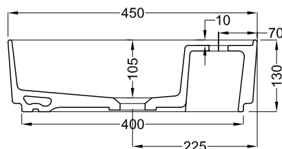
B - B SECTION
