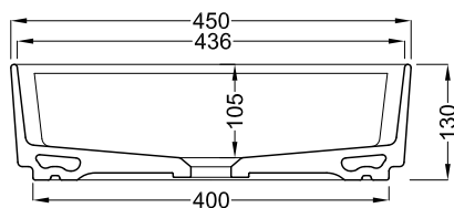
A - A SECTION
